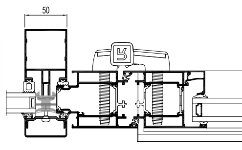
Integration into CW 50 façade
