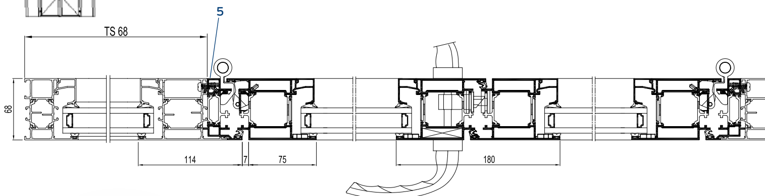
Composition with TS 68 structure and CD 68 2-vent door inward opening
